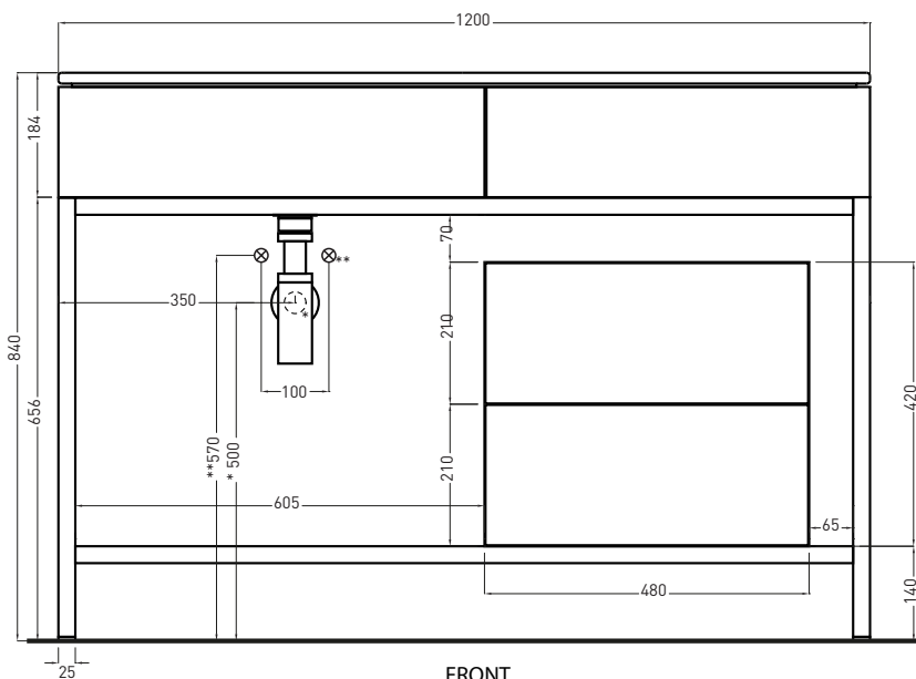
FRONT
