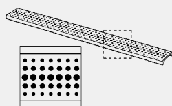
Advantix-Grătar Visign ER2 - inox 1.4301
